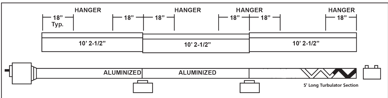
FIGURE 2D: Ener-Radiant XL Model ERXL-100 Assembly Overview
