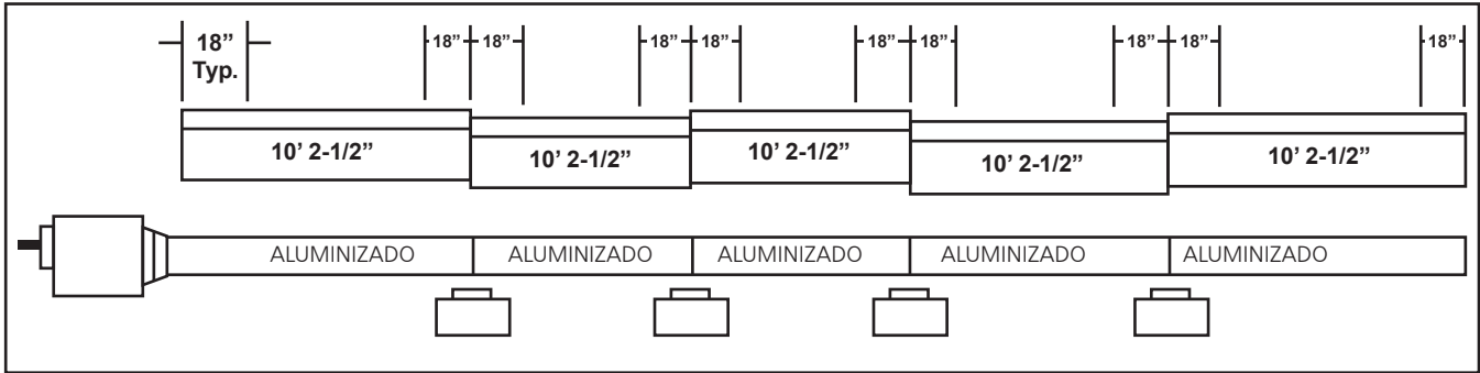
FIGURE 2G: Ener-Radiant XL Model ERXL-150, ERXL-175
