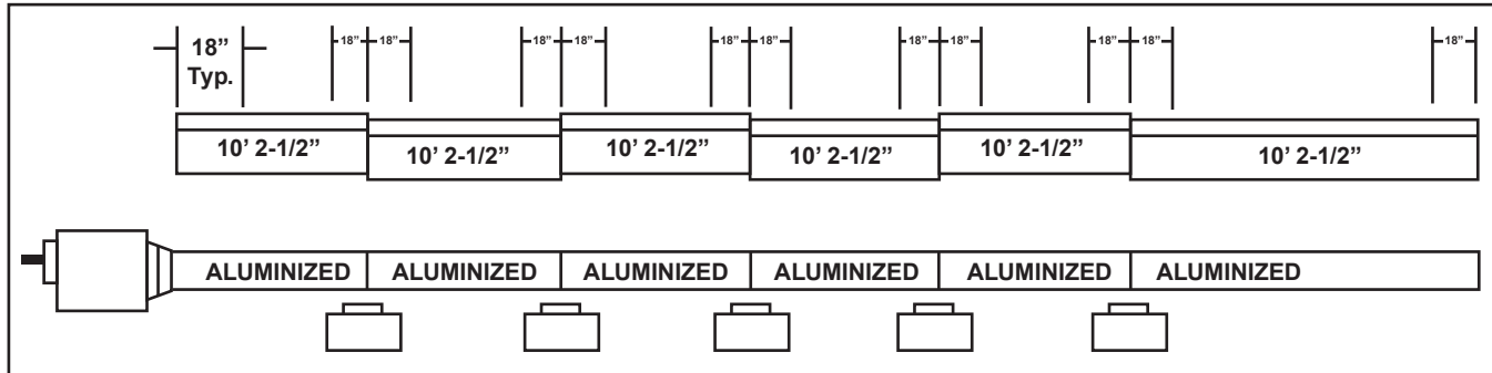
FIGURE 2G: Ener-Radiant XL Model ERXL-150, ERXL-175
