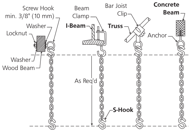
FIGURE 6: Typical Suspension Details
