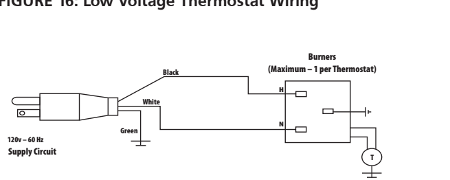
FIGURE 16: Low Voltage Thermostat Wiring
