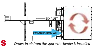
Draws in air from the space the heater is installed
